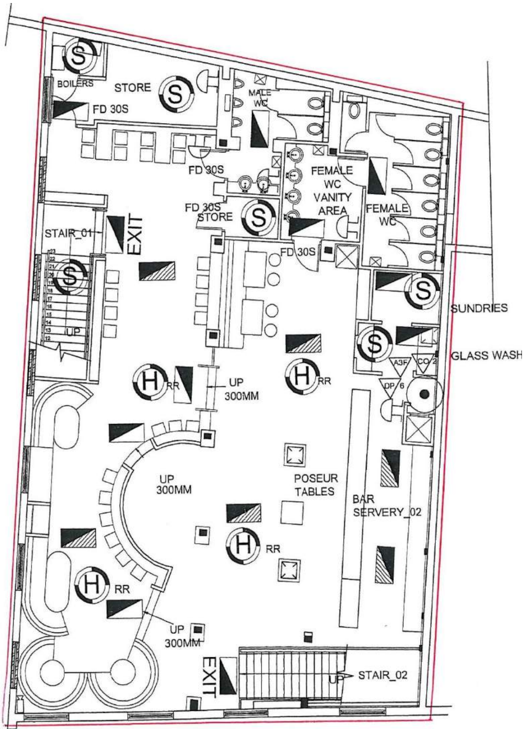
PROPOSED FIRST FLOOR LAYOUT
