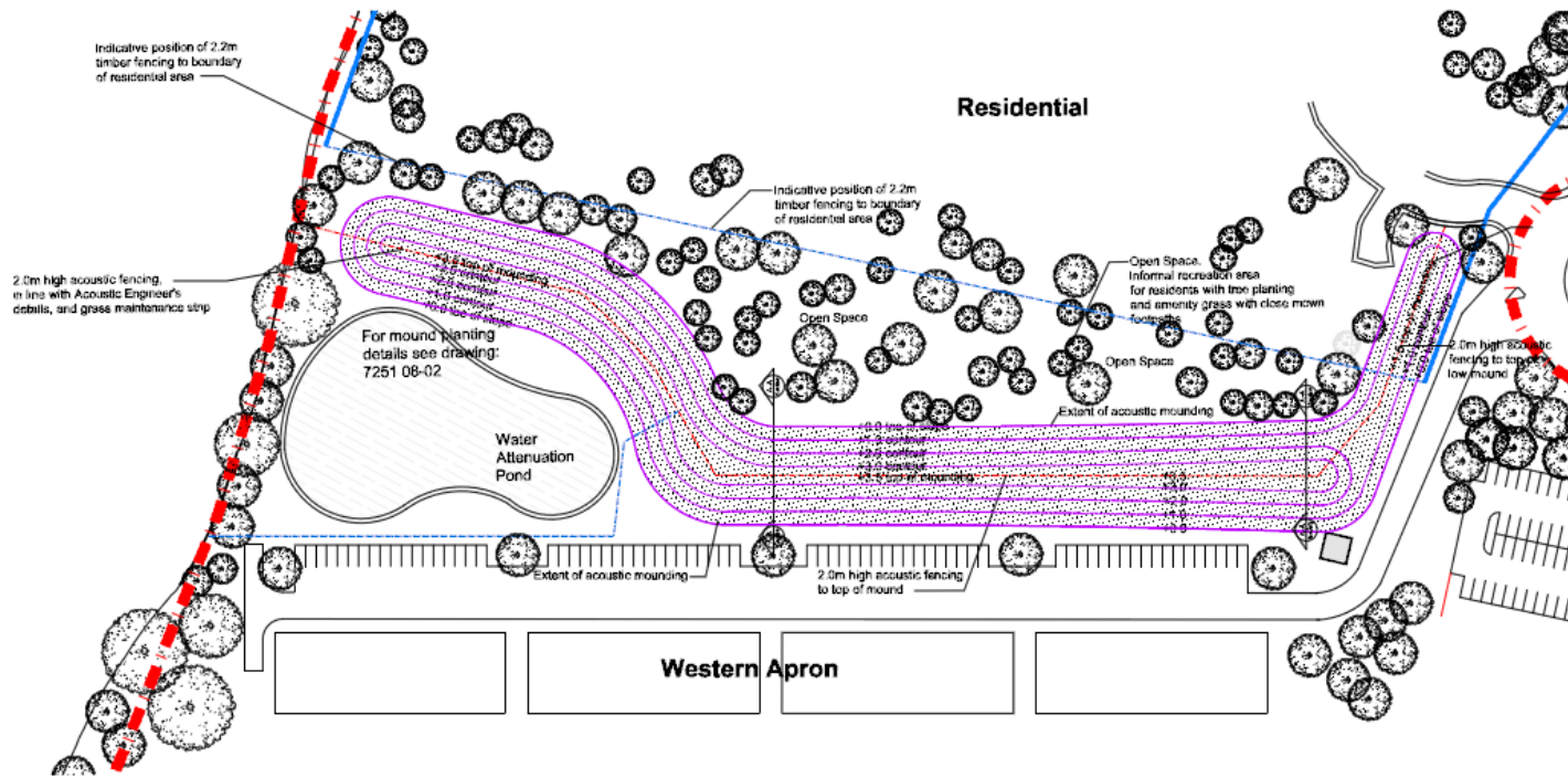
Acoustic Mounding GA 1:500
